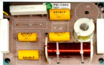
Ultra-linear Crossover Design
