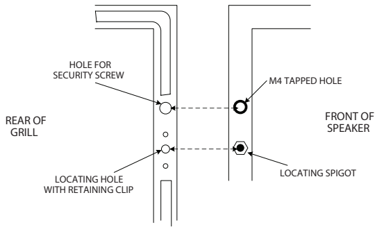
fig.11 - Securing the front grill
