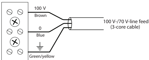
fig.8.2 - Wiring details B
