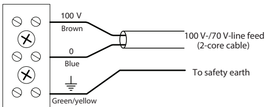
fig.8.1 - Wiring details A
