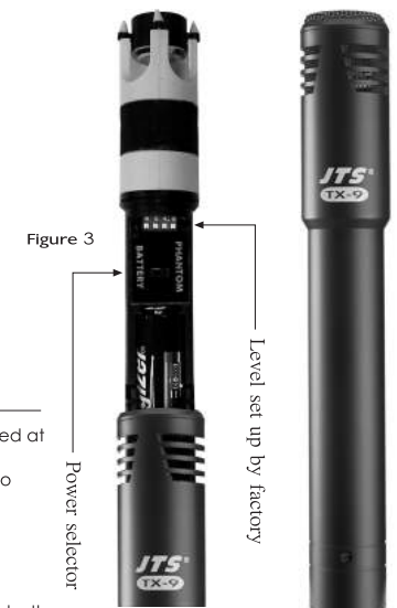
Instrument Condenser Microphone
