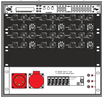
DASnet rack (2 patch panels + power distro 32Amp) (European version)
