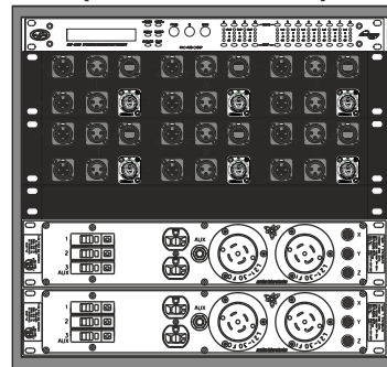
DASnet rack (2 patch panels + power distro 32Amp) (American version)
