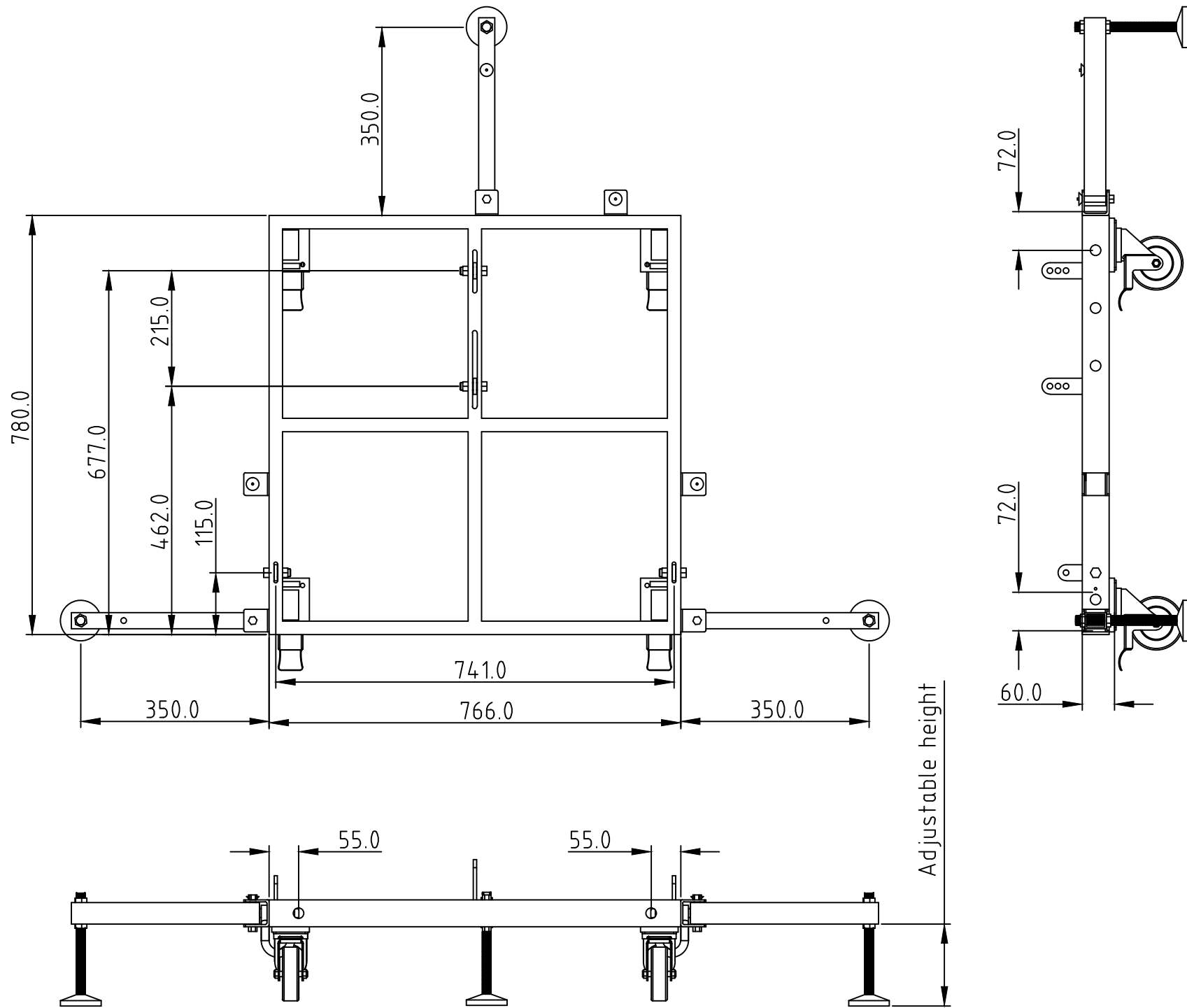
WLA-28 Dolly Frame
